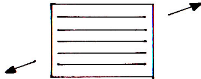
Figure 4-3 Example: Unidirectional composite (transversely isotropic)
