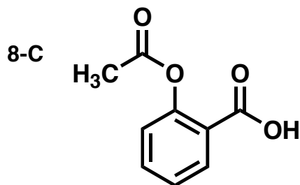
o -acetoxybenzoic acid aspirin
