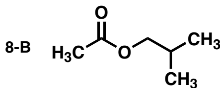
isobutyl acetate bananas
