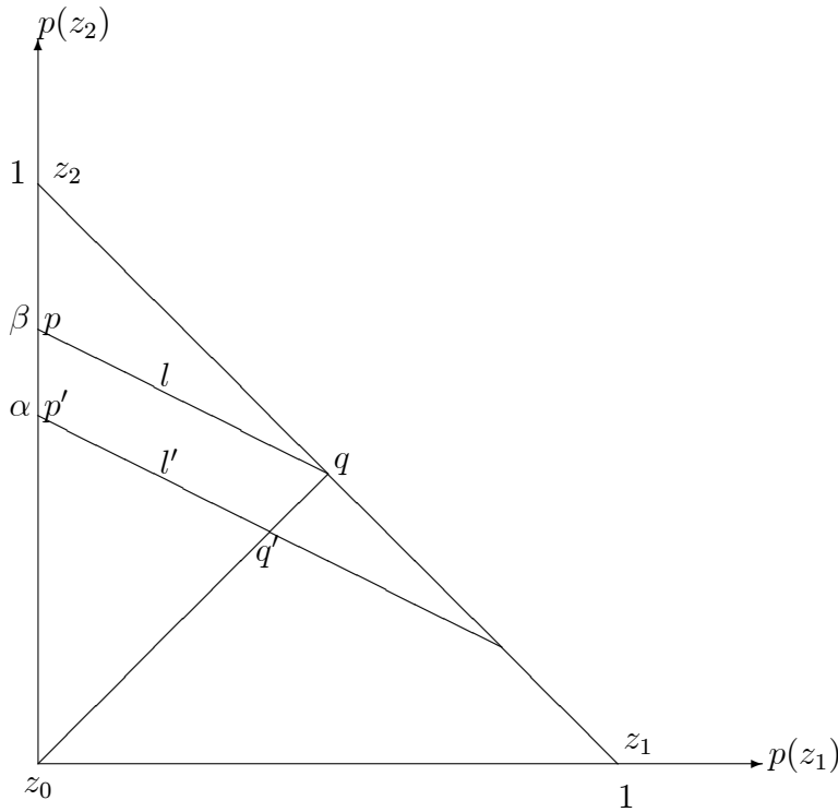
Figure 2.3: Indifference curves on the space of lotteries
