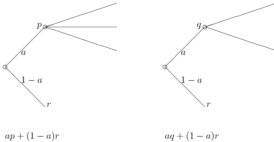
Figure 2.2: Two compound lotteries
